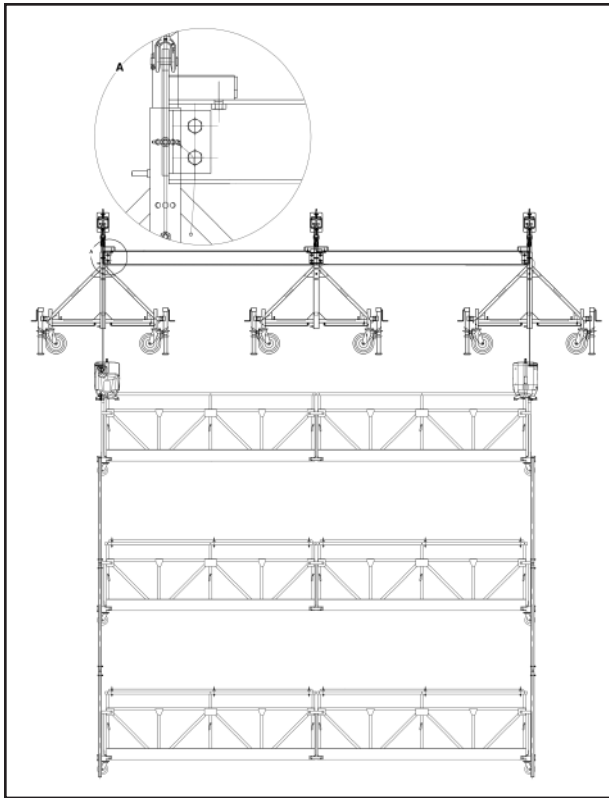
Multi-level platform & rigging
