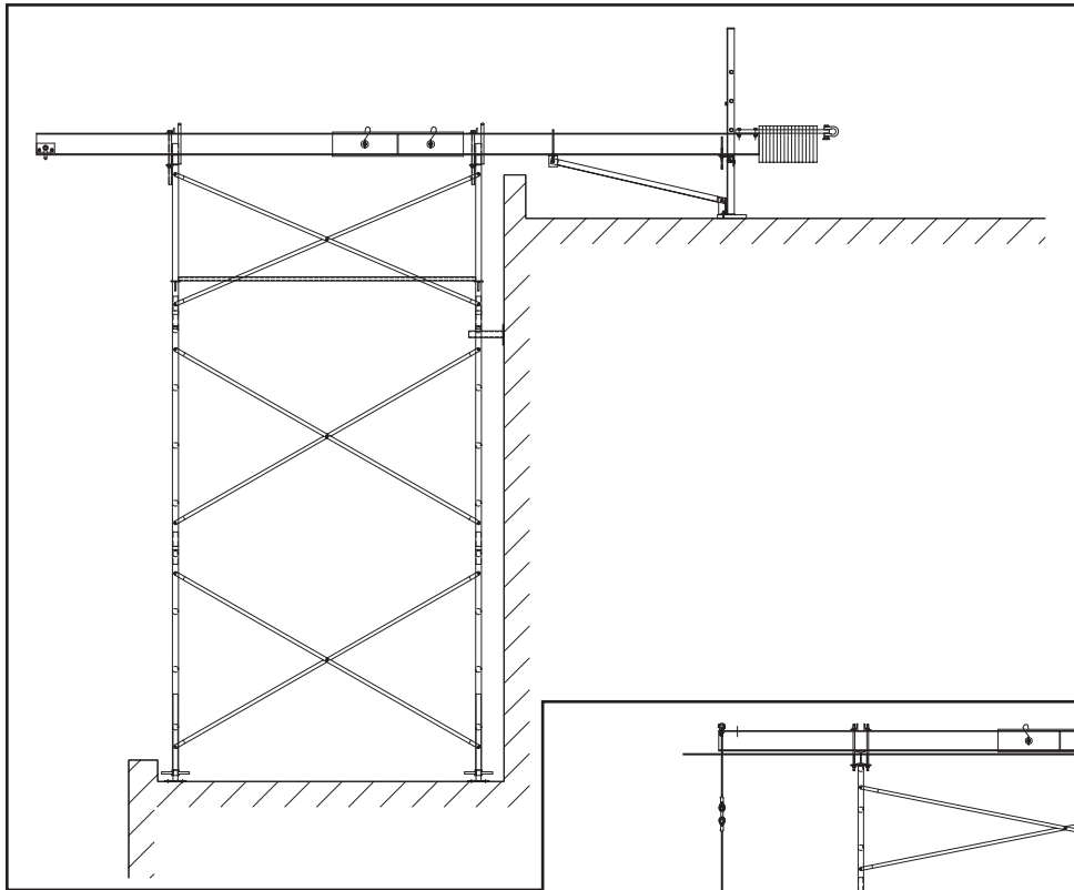
Outrigger tower in small space
