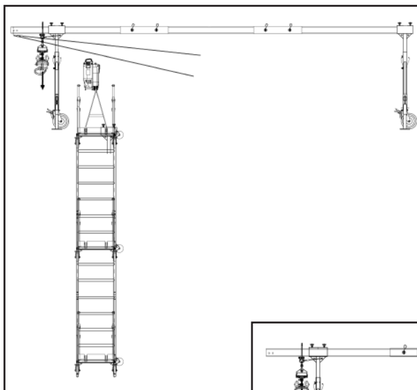
Multi-level platform & rigging
