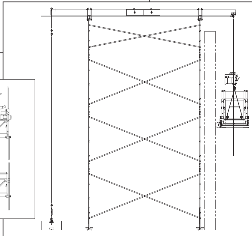
Outrigger beam on scaffold towers
